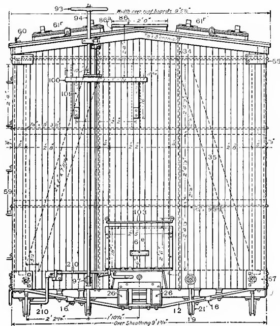
Fig. 280. End Elevation.
